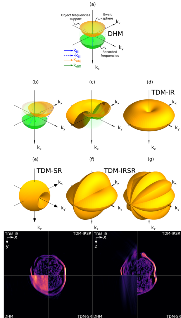
Figure 22. Optical Transfer Function (OTF) for various configurations in transmission TDM. a) Digital holographic microscopy: the OTF depicts a cap of sphere with large lateral, but limited longitudinal extension. b) With inclined illumination, same positions of \mathbf{k}_{\text{diff}} vectors provide new \mathbf{k}_{\text{obj}} vectors. c, d) With many illuminations, a filled, extended OTF is obtained. e) With sample-rotation, an almost completely filled sphere is obtained (but of lesser extension than in previous case). f, g) OTFs combining illumination and sample rotation with 2, and 4 evenly spaced specimen positions. Bottom row: Betula pendula pollen grain images in DHM and three TDM variants. Left composite image depicts x-y slice in the focal plane, showing improved resolution in TDM, but only twice that of DHM. Contrast is however better thanks to better optical sectioning. Right composite image highlights the large differences in imaging capabilities along the optical axis. Only TDM-IRSR can deliver true improved and isotropic resolution, while holography is not, strictly speaking, a true 3-D imaging method when considering transparent samples: only optical thickness can be measured.
