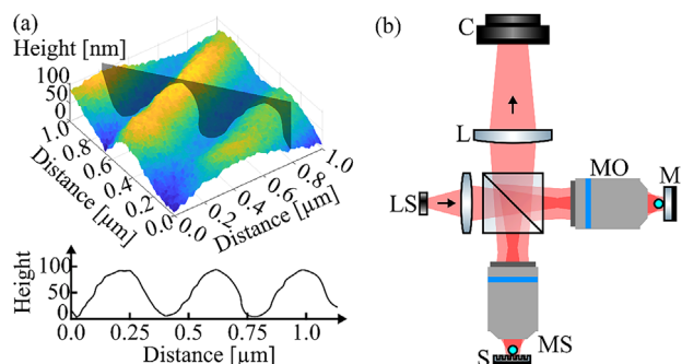
Figure 54. a) Surface topography reconstructions of a 200-nm-groove standard and b) layout of compensated microsphere-assisted interference microscope. LS, light source. MO, microscope objective. MS, microsphere. S, sample. M, reference mirror (with a microsphere). L, relay lens. C, camera.
