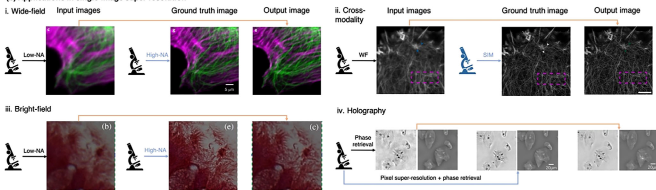
Figure 5. Applications of DL-SR optical microscopy. a) STORM, [160] SIM, [191] PALM, [187] and Fourier ptychographic microscopy (FPM). [194] b) Single-image super-resolution in wide-field fluorescence, [172, 174] bright-field, [55] and digital holographic microscopy. [195] Reproduced with permission. [55, 160] Copyright 2017 and 2018, The Optical Society.
