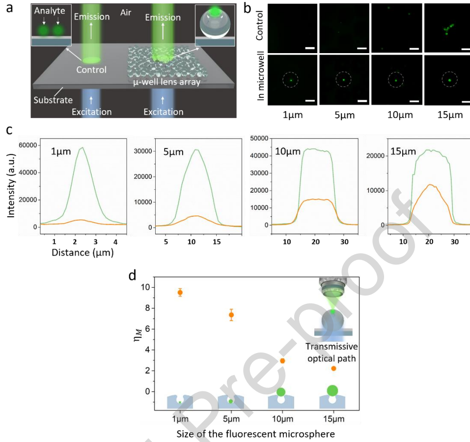
Figure 3. (a) Schematic illustration of the signal recording for the fluorescent microspheres in the semi-open microwells and on the substrate (control) and (b) corresponding recorded fluorescent signals. (c) The fluorescent intensity from the corresponding fluorescent microspheres showing the enhanced fluorescent signal (green curve) and the control signal (orange curve). (d) The enhancement factor v.s. the size of the fluorescent microspheres measured by experiment (error bar stands for standard deviation).
