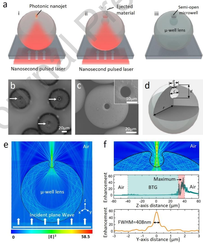
Figure 1. Fabrication and characterization of the \mu -well lens. (a) Schematic
