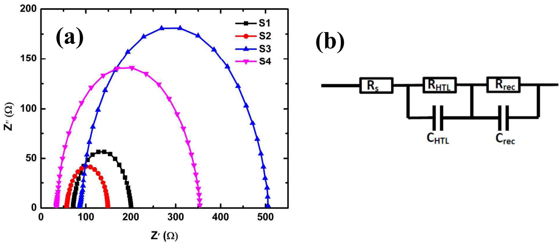
Fig. 4 (a) Nyquist plots of devices based on p-TiO 2 without and with Au NP and MgO coating under dark condition at 0.9 V applied bias. (b) Simplified equivalent circuit to fit the impedance spectra.
